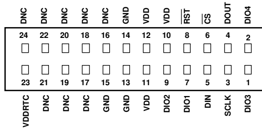
ADIS16480 TOP VIEW (Not to Scale)
