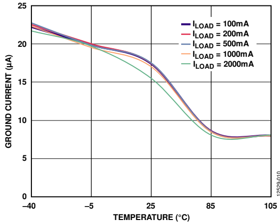
Figure 10. Ground Current vs. Temperature, Different Load Currents, V_{IN} = 13.2V
