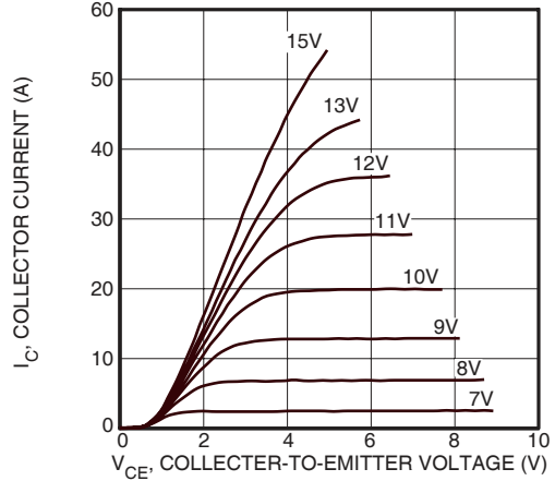
FIGURE 2, Output Characteristics ( T_J = 125^\circ C )
