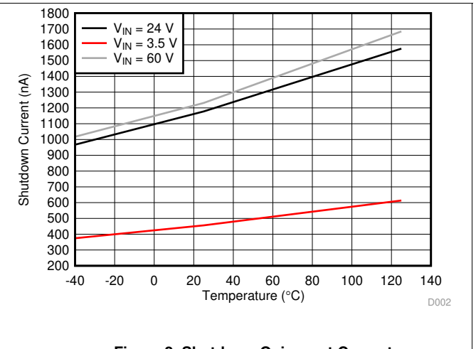
Figure 2. Shutdown Quiescent Current
