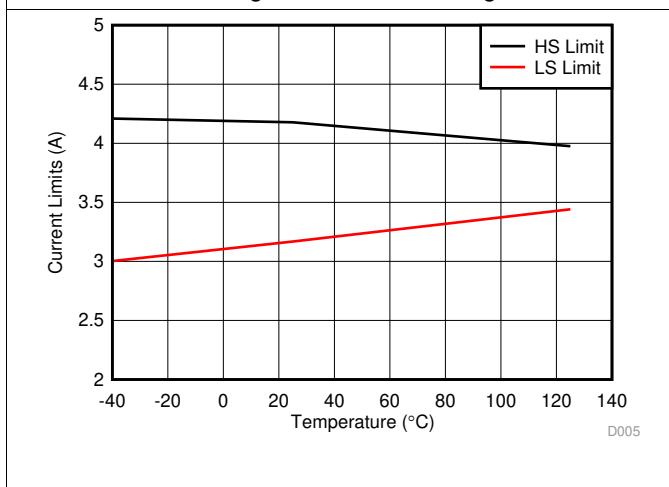
Figure 5. LM76002 High-Side and Low-Side Current Limits
