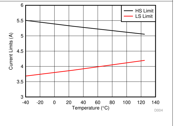
Figure 4. LM76003 High-Side and Low-Side Current Limits
