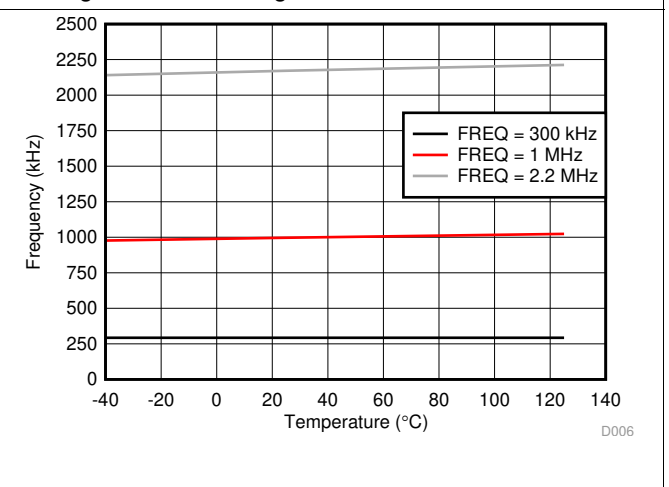
Figure 6. Switching Frequency Set by R T Resistor
