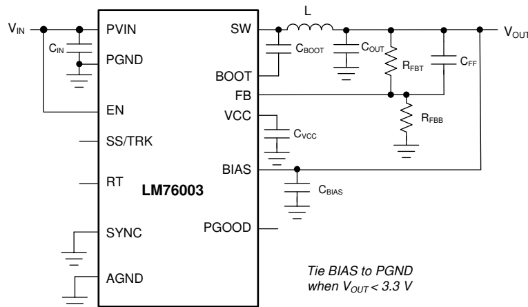
Figure 21. LM76002/LM76003 Basic Schematic
