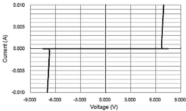
Fig 3 Voltage Sweeping
