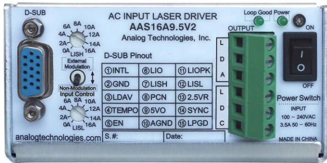
Figure 1. Front View of the AAS16A9.5V2
