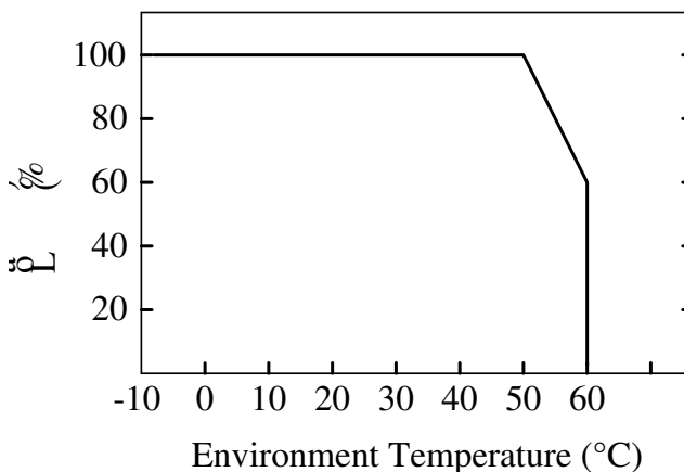
Figure 26. Derating Curve
