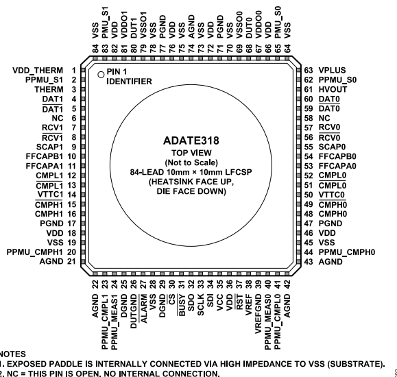
Figure 8. LFCSP Pin Configuration
