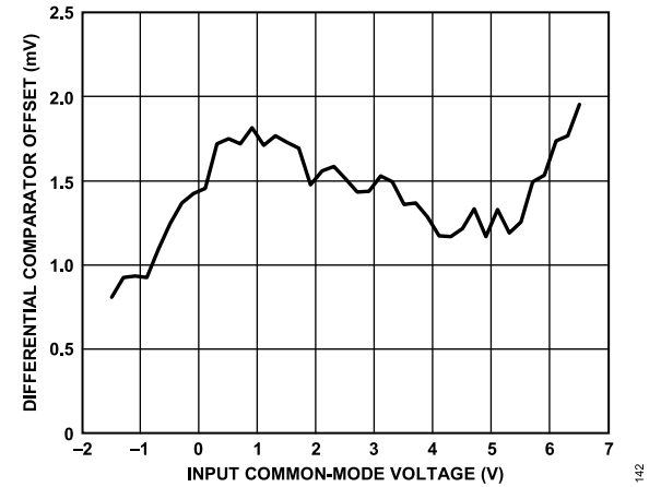
Figure 49. Differential Comparator CMR Error
