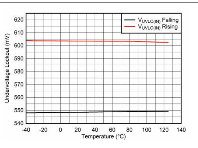
Figure 6-12. V_{\text{IN}} UVLO vs Temperature
