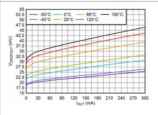
Figure 6-4. V_{\text{IN}} Dropout Voltage vs I_{\text{OUT}}
