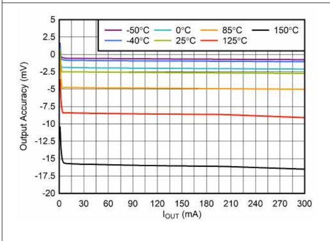
Figure 6-3. Output Voltage Accuracy vs I_{\text{OUT}}
