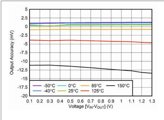
Figure 6-1. Output Voltage Accuracy vs V_{\text{IN}}
