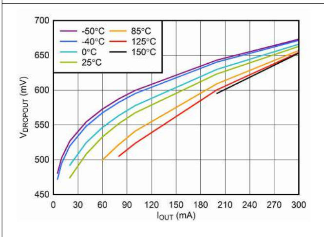
Figure 6-5. V_{\text{BIAS}} Dropout Voltage vs I_{\text{OUT}}
