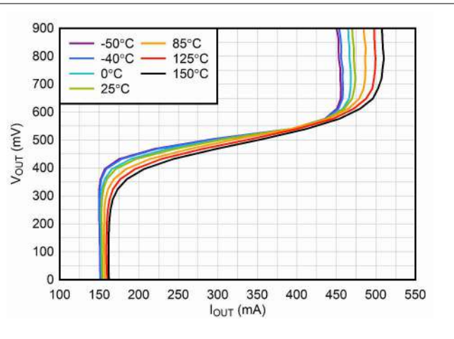
Figure 6-10. Foldback Current Limit vs I_{\text{OUT}}
