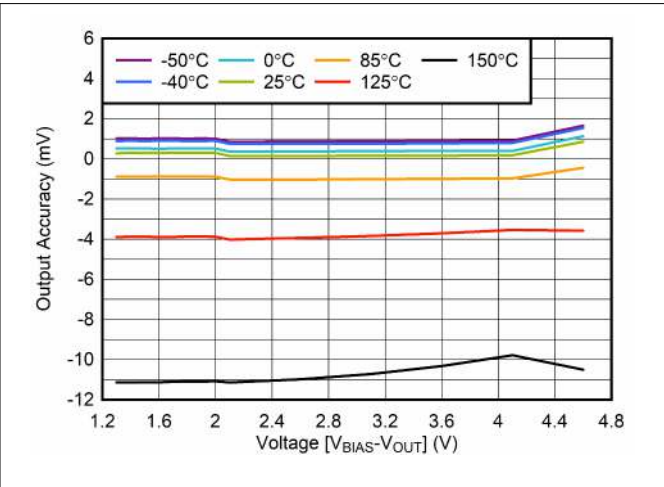
Figure 6-2. Output Voltage Accuracy vs V_{\text{BIAS}}
