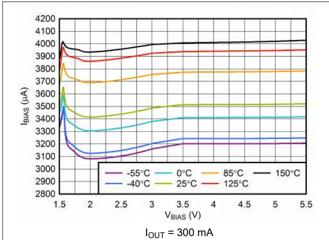
Figure 6-7. V_{\text{BIAS}} Input Current vs V_{\text{BIAS}}
