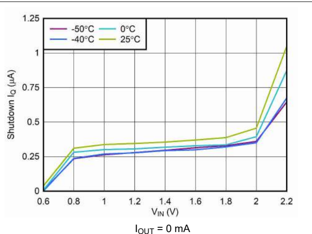
Figure 6-8. V_{\text{IN}} Shutdown I_Q vs V_{\text{IN}}
