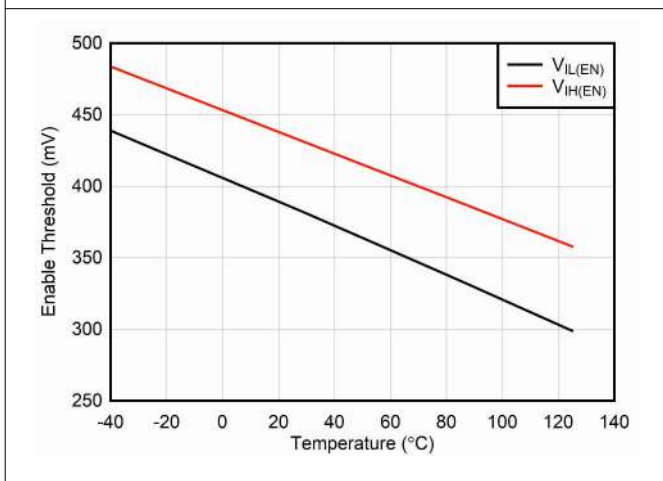
Figure 6-11. Enable Threshold vs Temperature
