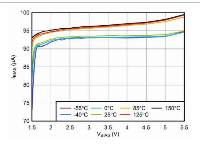
Figure 6-6. V_{\text{BIAS}} Input Current vs V_{\text{BIAS}}
