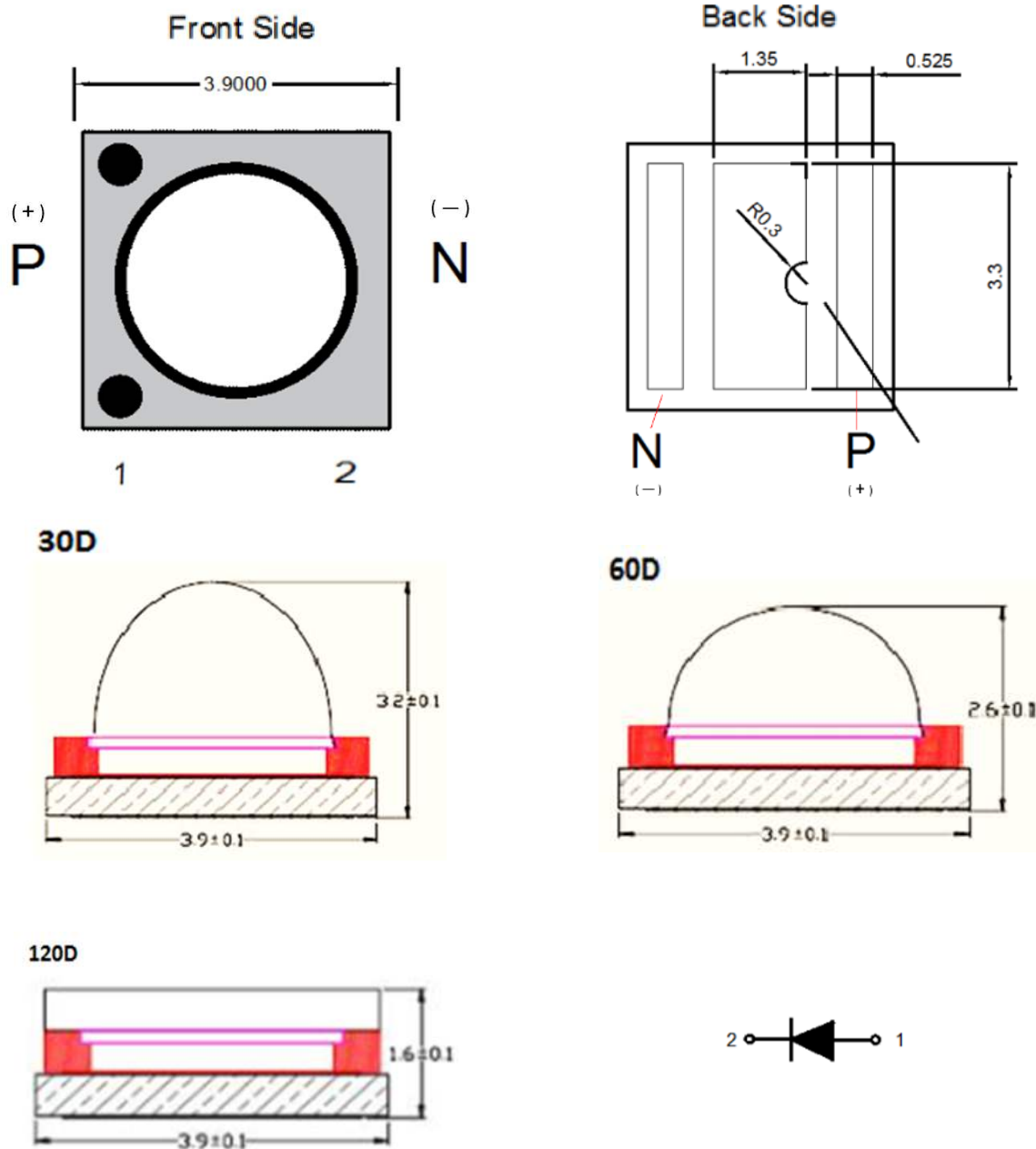
Figure 2. IN-C40PU(X)TK UVC series Package Dimension
