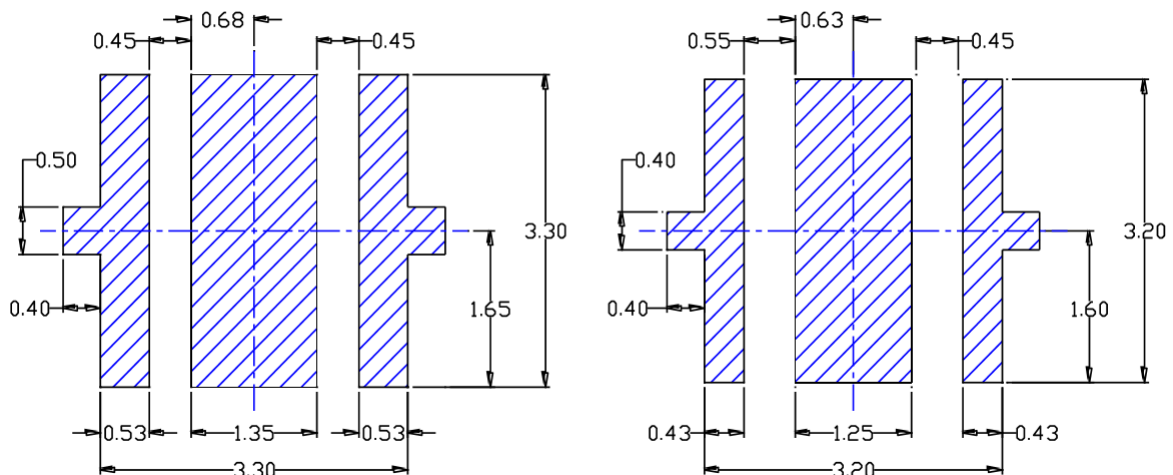
Figure 1. IN-C40PU(X)TK UVC series Recommended Solder Pattern
