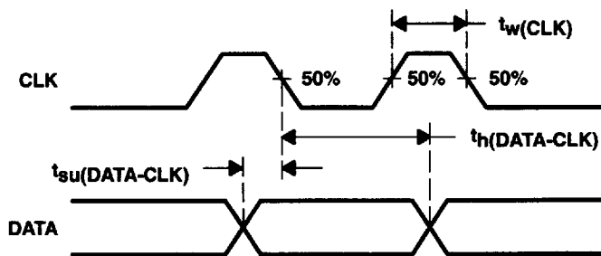
Figure 6. Timing of DATA Relative to CLK
