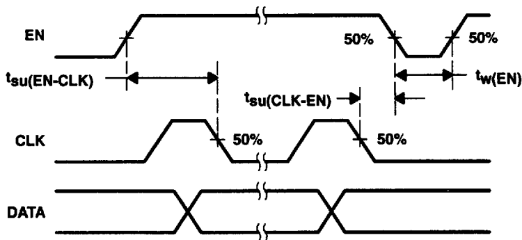
Figure 7. Timing of CLK Relative to EN
