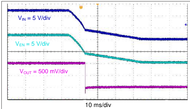
Figure 34. TPS563201 Shutdown Relative to V_I
