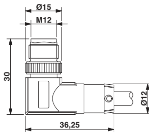
Dimensioned drawing
