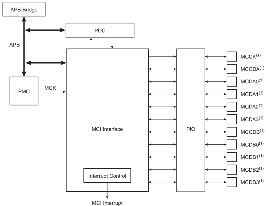
Figure 33-1. Block Diagram
