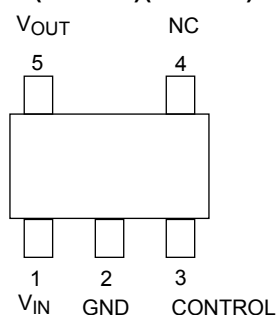
SMV(SOT-25)(SC-74A)
