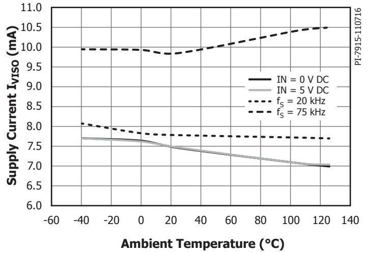
Figure 16. Supply Current Secondary-Side I_{VISO} vs. Ambient Temperature. Conditions: V_{VCC} = 5\text{ V} , V_{TOT} = 25\text{ V} , No-Load.
