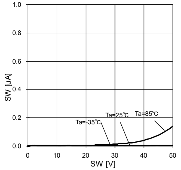
Fig.17 SW Leak Current
