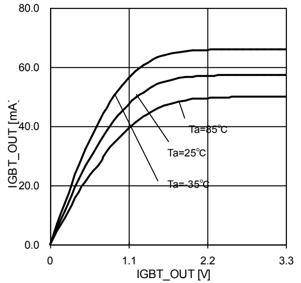
Fig. 23 IGBT_OUT Sink Current
