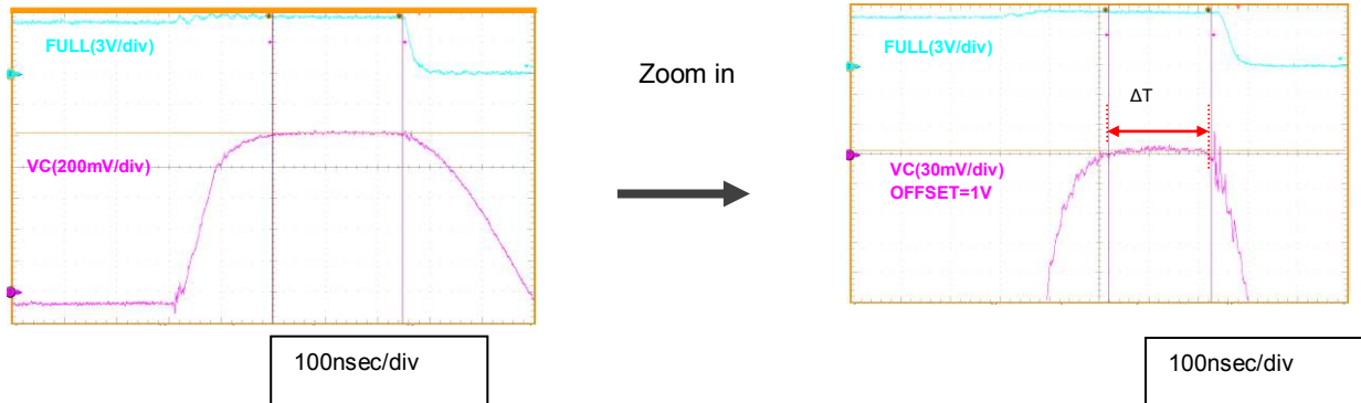
Fig42. Setup of VC pin voltage to flat
