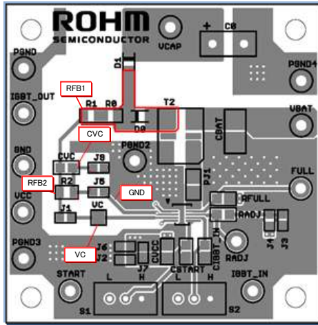
Fig35. PCB layout pattern of board
