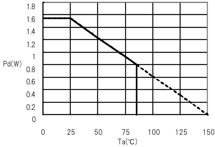
Fig 49. Heat reduction characteristics (VSON010V3020)
