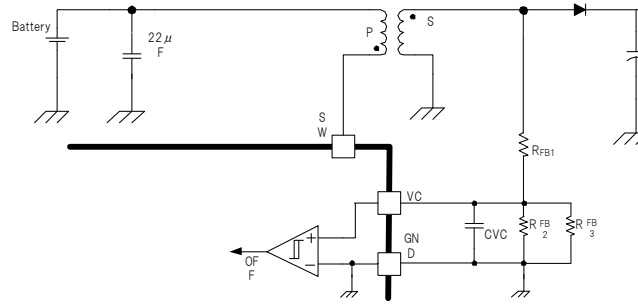
Fig 34. VC pin external parts
