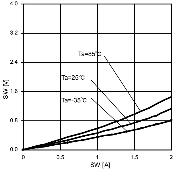
Fig.16 SAT Voltage
