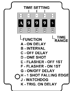
Figure 1 - Multi-Function (TD-781)
