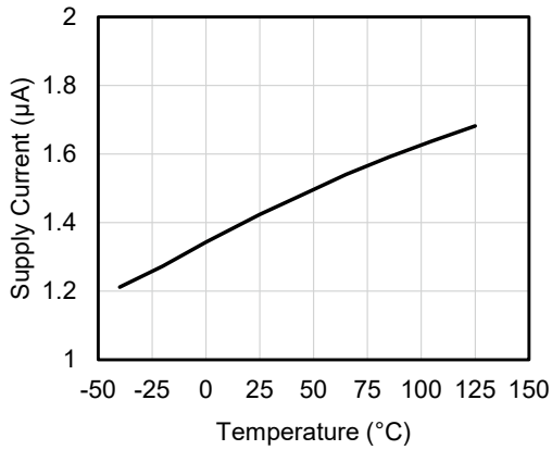
Figure 19. Supply current versus temperature (V cc = 3 V)
