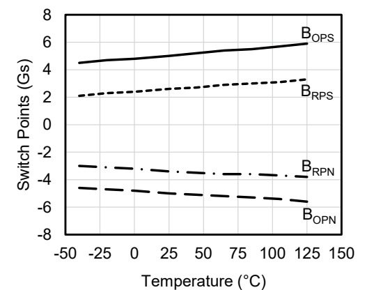
Figure 22. Switch points versus temperature (V cc = 3 V)
