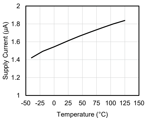
Figure 21. Supply current versus temperature (V cc = 3 V)
