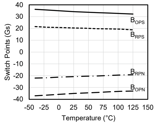
Figure 18. Switch points versus temperature (V cc = 3 V)
