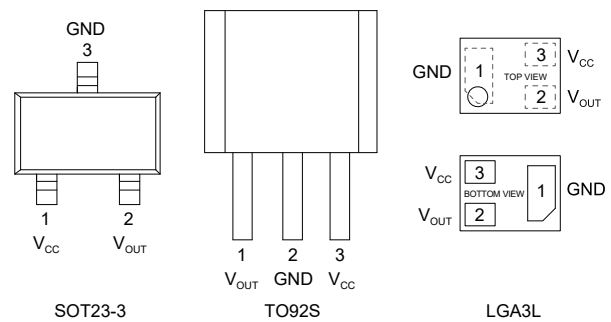
Figure 4. Pin configuration
