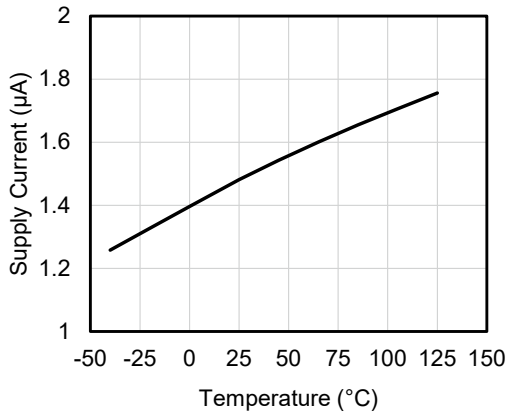
Figure 17. Supply current versus temperature (V cc = 3 V)
