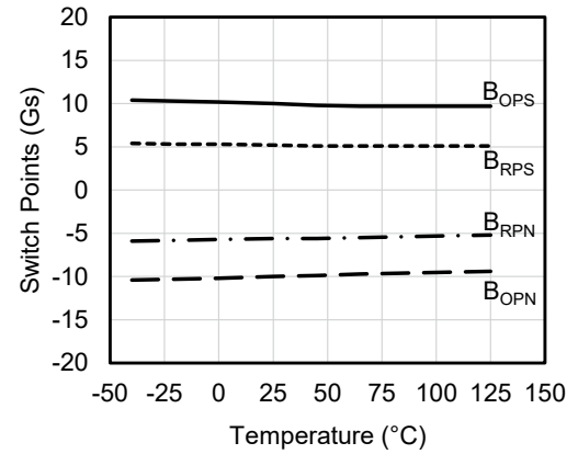
Figure 20. Switch points versus temperature (V cc = 3 V)
