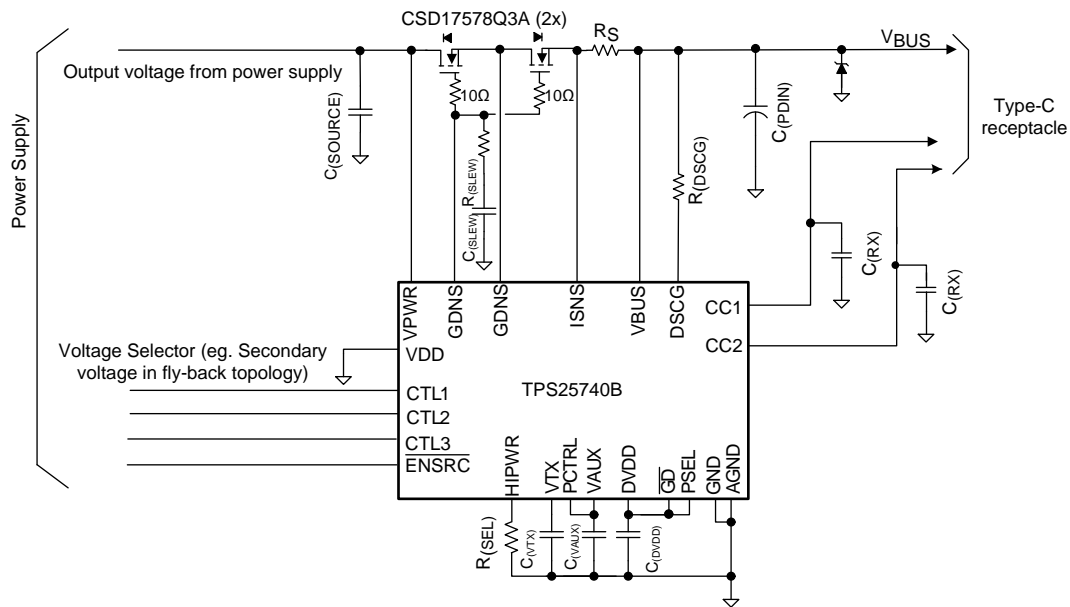
Figure 21. Schematic 1
