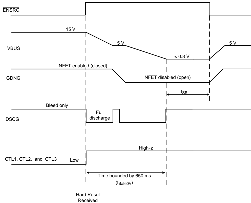
Figure 7. Timing Diagram for \overline{ENSRC} and GDNG After Receiving a Hard Reset
