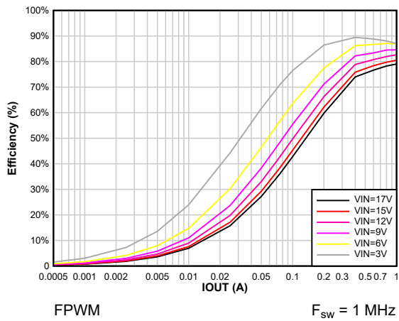
Figure 8-7. Efficiency vs Output Current V_{OUT} = 1.2 \text{ V}
