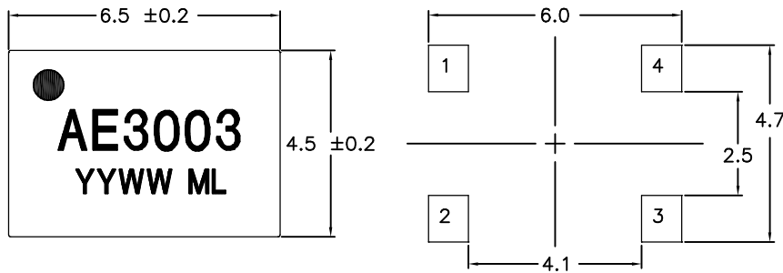
RECOMMENDED FOOTPRINT
