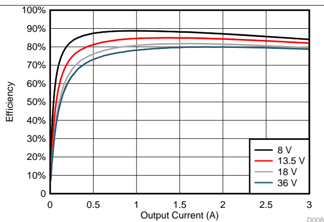
Figure 8. Efficiency (LM536033, FPWM Mode)
