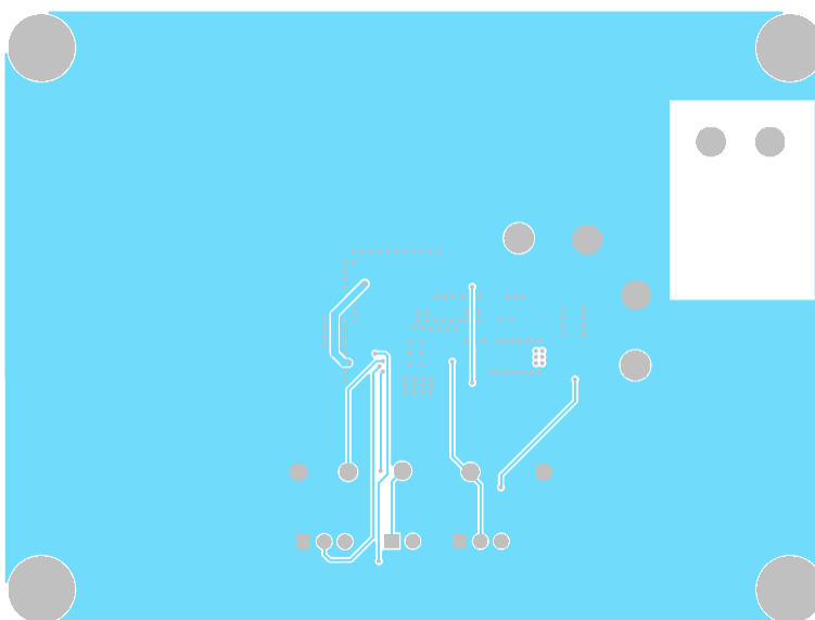
Figure 5-3. Mid Layer 2
