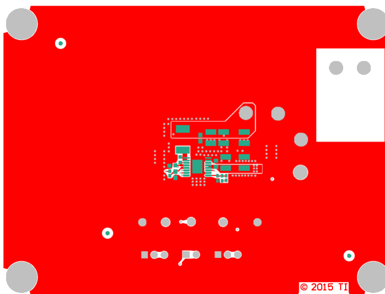
Figure 5-1. Top Layer
