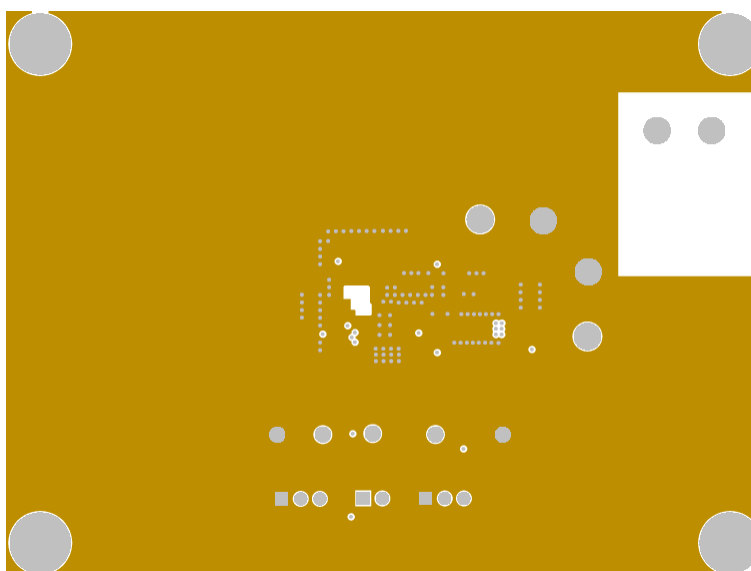
Figure 5-2. Mid Layer 1
