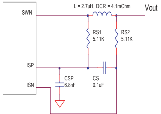
Figure 1: Over-current detection circuit
