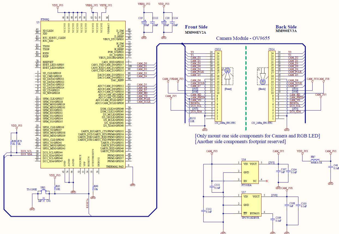
Figure 4-12 – Camera connector
