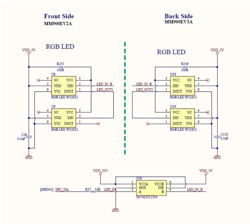
Figure 4-13 – RGB LEDs
