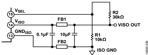
Figure 31. V_{ISO} Bias and Bypass Components
