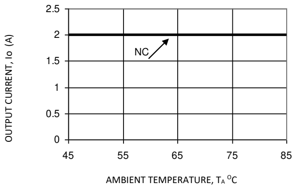
Figure 11. V_o = 3.3 V
