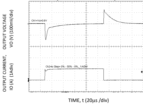
Figure 19. Transient Response to Dynamic Load Change from 0% 50% to 0%. V_o = 0.6\text{ V}
