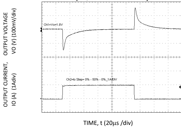
Figure 21. Transient Response to Dynamic Load Change from 0% 50% to 0%. V_o = 1.6\text{ V}
