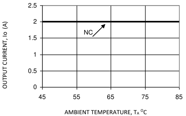
Figure 12. V_o = 5.0 V
