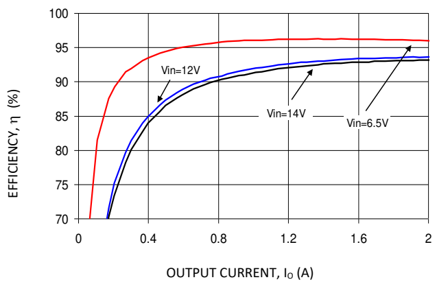
Figure 6. V_o = 5.0 V
