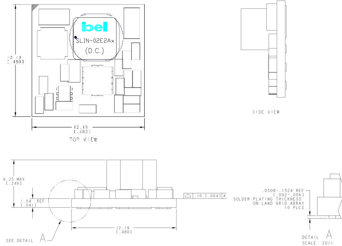
Figure 52. Outline
