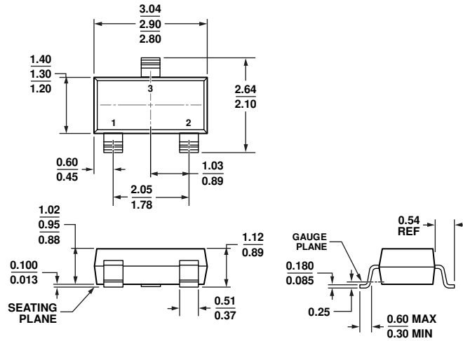
Figure 15. 3-Lead Small Outline Transistor Package [SOT-23] (RT-3)
