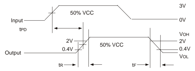
Figure 2. Voltage Waveforms Propagation Delay Times
