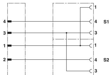
Contact assignment of the M12 Y-distributor
