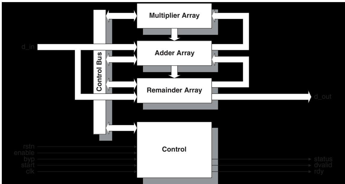
Figure 1. Reed-Solomon Encoder Core Block Diagram
