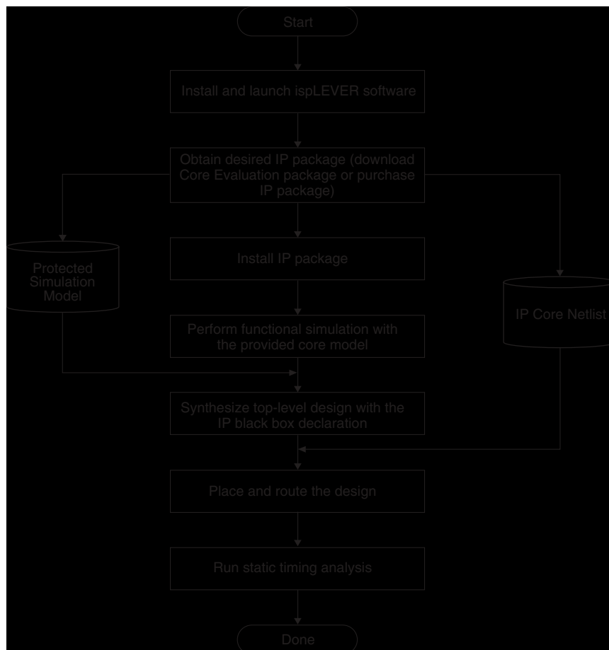
Figure 10. Lattice IP Core Implementation Flow
