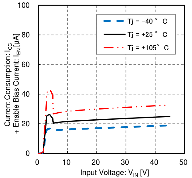
Figure 4. Current Consumption + Enable Bias Current vs Input Voltage
