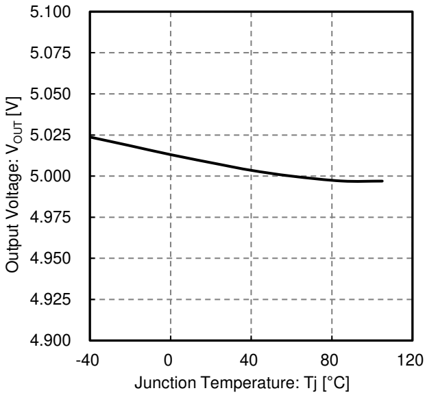
Figure 3. Output Voltage vs Junction Temperature ( I_{OUT} = 0.5\text{ mA} )
