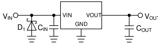
Figure 25. Surges Lower than -0.3 V is Applied to the Input
