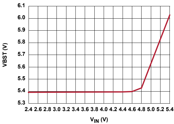
FIGURE 8. VBST, V_{IN} HEADROOM TRACKING, V_{BST} = 5.4\text{V}
