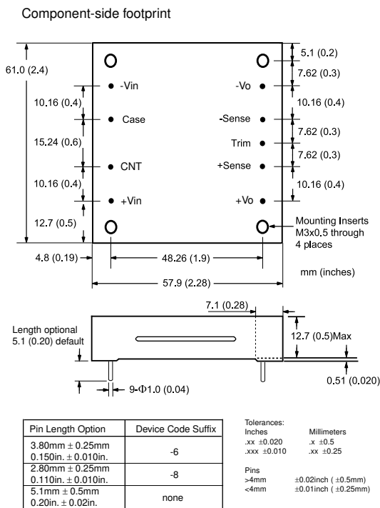
Fig.1 Dimensions
