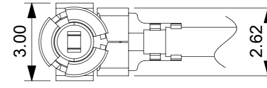
U.FL CONNECTOR
