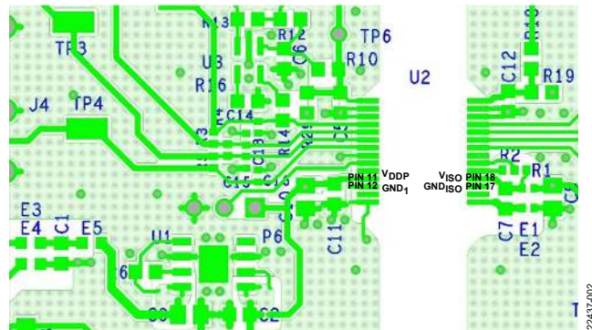
Figure 3. Layout Notes for EVAL-ADUM6421ARNZ/EVAL-ADUM6421AURNZ
