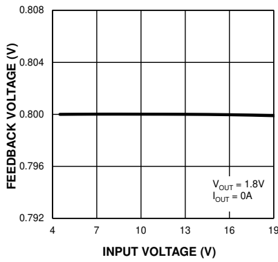
Feedback Voltage vs. Input Voltage
