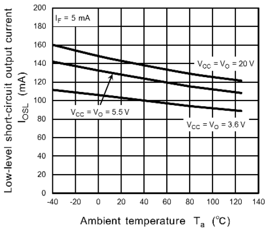
Fig. 12.2.9 I_{osL} - T_a
