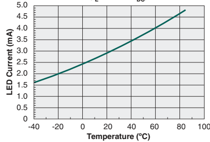
Typical I_F for Switch Dropout vs. Temperature ( I_L=200mA_{DC} )
