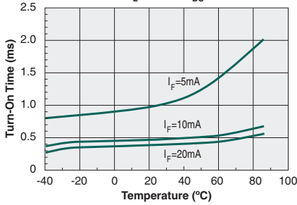
Typical Turn-On Time vs. Temperature ( I_L=200mA_{DC} )
