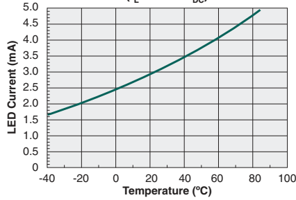
Typical I_F for Switch Operation vs. Temperature ( I_L=200mA_{DC} )
