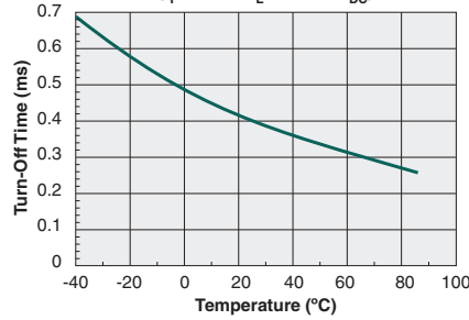
Typical Turn-Off Time vs. Temperature ( I_F=5mA, I_L=200mA_{DC} )
