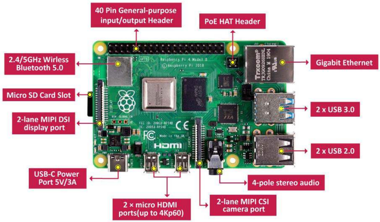
Raspberry Pi 4 Hardware Overview by Seed
