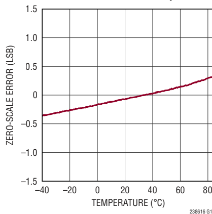
Zero-Scale Error vs Temperature
