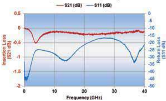
P21BN300MA4572 Opti-Cap Typical Performance (Reference 50 Ohm System)
