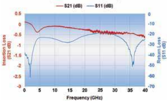
P21BN300MA04733 Opti-Cap Typical Performance (Reference 50 Ohm System)
