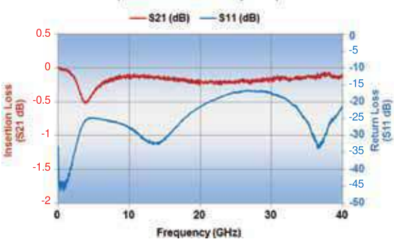
P42BN300MA4679 Opti-Cap Typical Performance (Reference 50 Ohm System)
