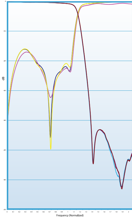
Lowpass Filter - 3 Samples
