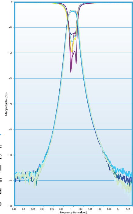
Cavity Filter - 5 Samples
