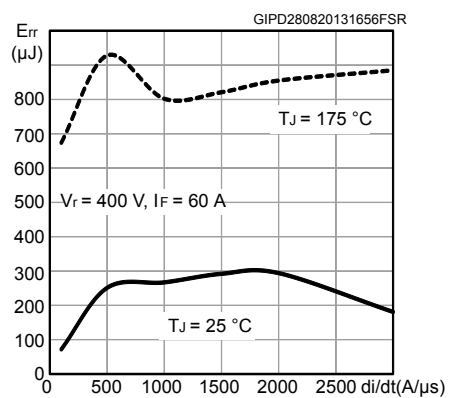
Figure 24. Reverse recovery energy vs. diode current slope
