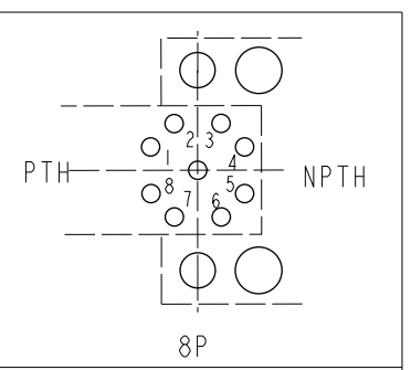
Pin Definition
