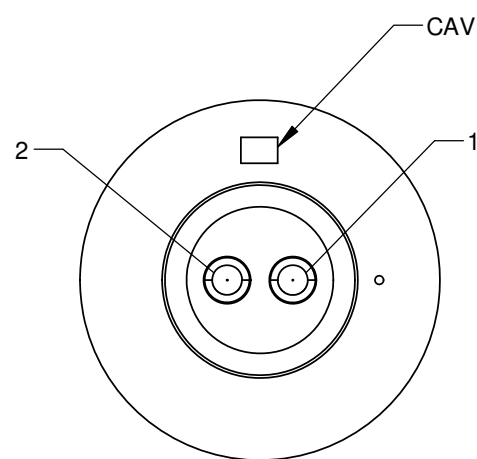
WIRE VIEW 17282-2PG-00
