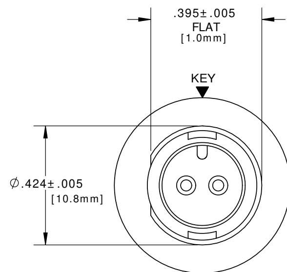
FACE VIEW
