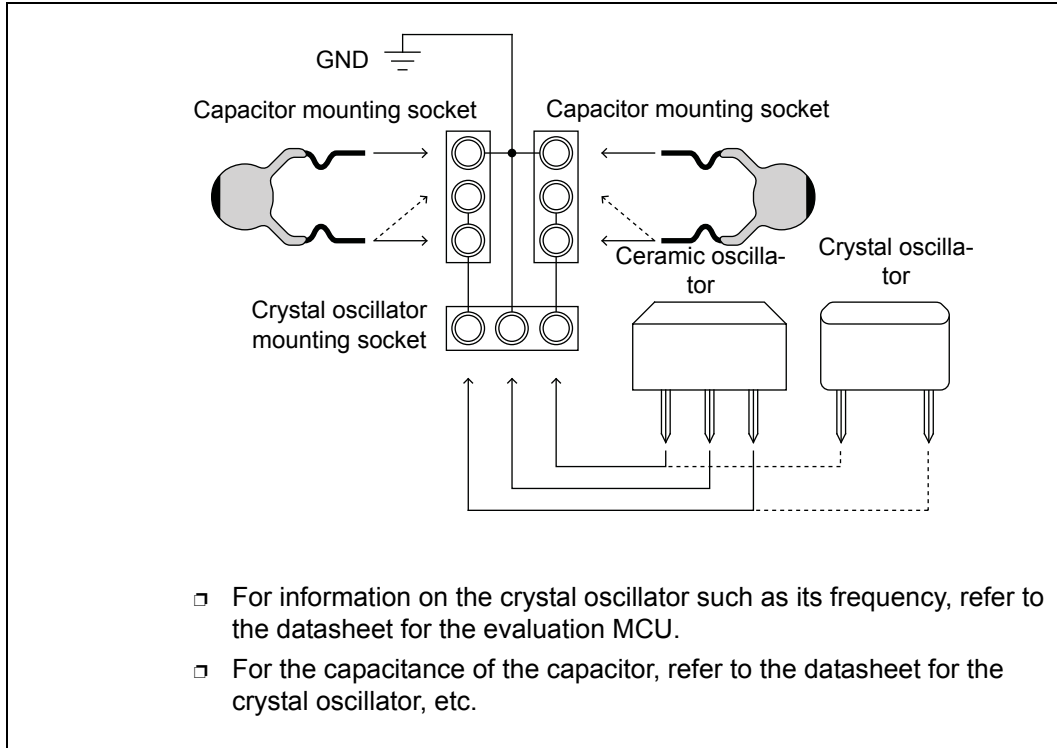
Figure 4-2. The Example of Mount of Crystal or Ceramic Oscillator
