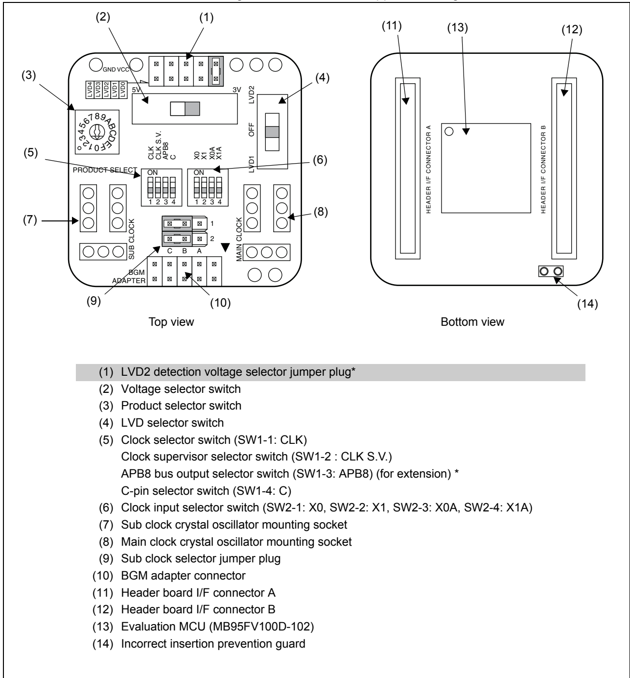
Figure 1-2. MCU Board Appearance Figure
