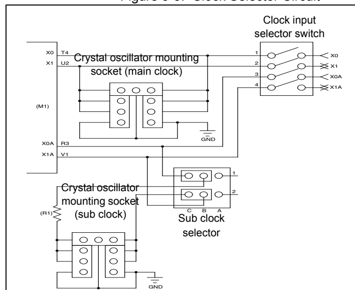
Figure 5-3. Clock Selector Circuit
