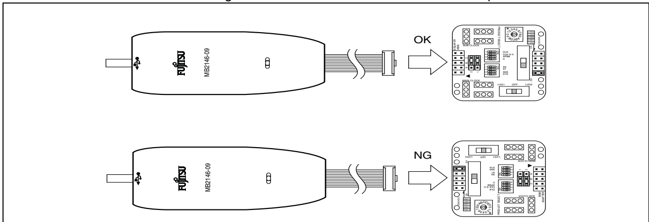
Figure 3-3. Connection Direction of BGM Adapter
