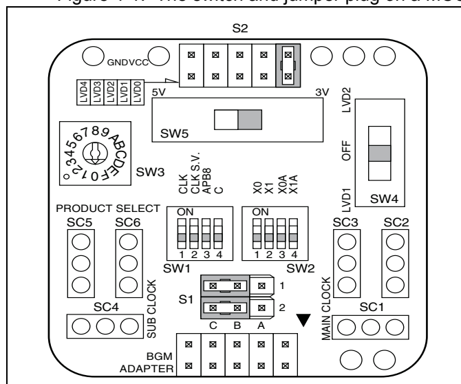
Figure 4-1. The switch and jumper plug on a MCU board
