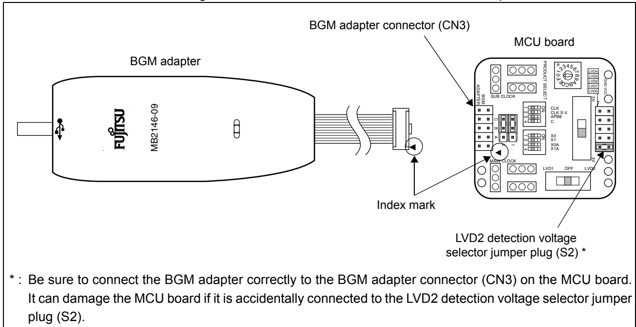
Figure 3-2. Connection of MCU Board and BGM Adapter
