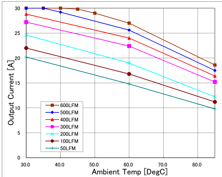
Fig-1: Available load current vs. ambient temperature and airflow rates for Vin=48V. Maximum component temperature \leq 125^{\circ}\text{C}
