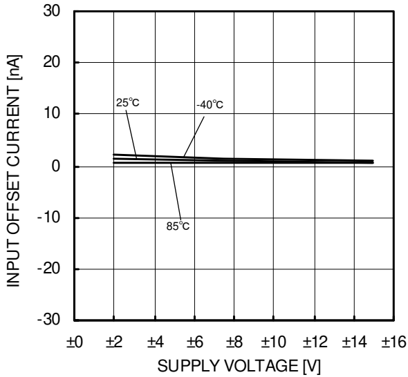
Fig.14 Input Offset Current - Supply Voltage (V icm =0V, V out =0V)
