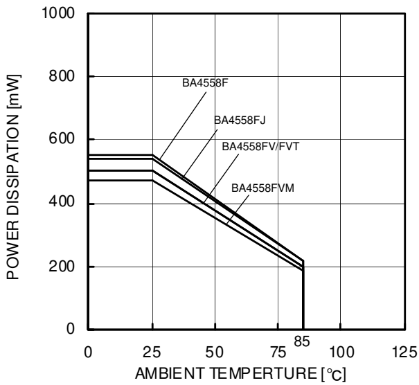
Fig.2 Derating Curve
