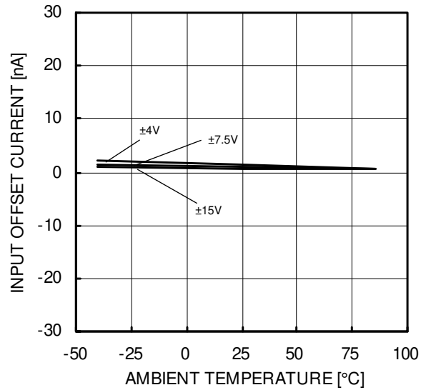
Fig.15 Input Offset Current - Ambient Temperature (V icm =0V, V out =0V)
