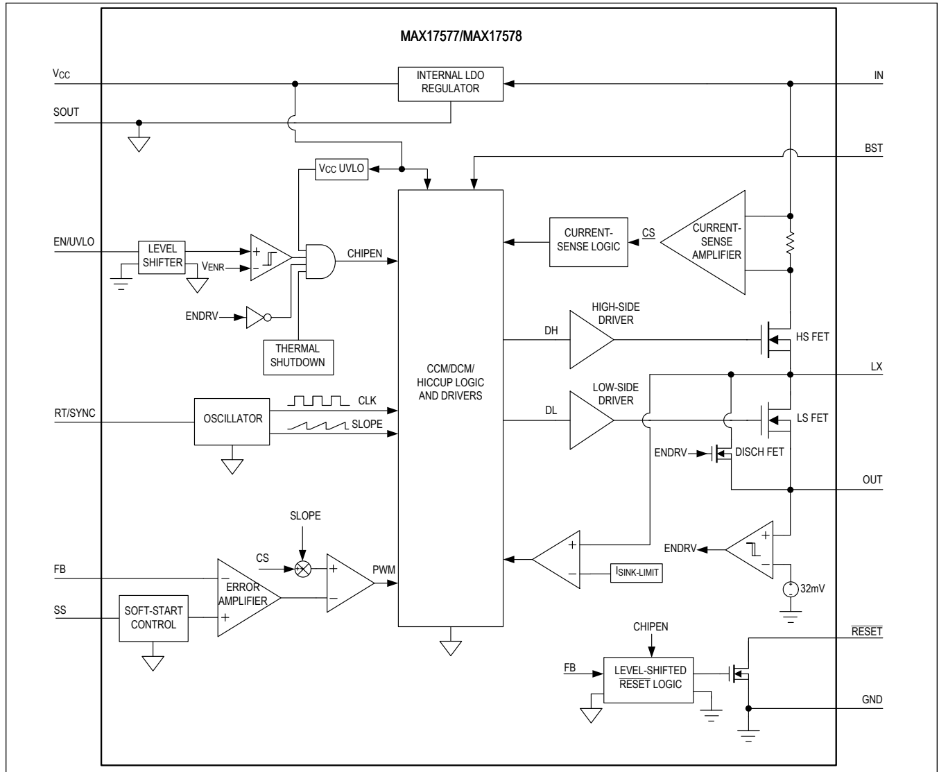
MAX17577/MAX17578 Block Diagram
