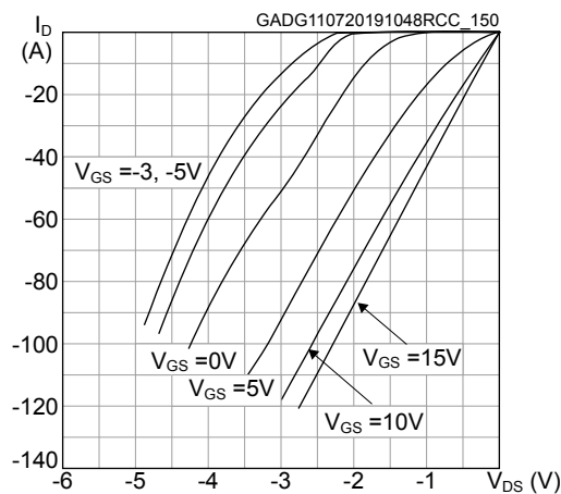
Figure 17. Typical reverse conduction characteristics ( T_J = 150\ ^{\circ}\text{C} )
