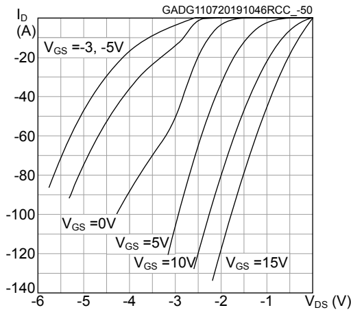
Figure 15. Typical reverse conduction characteristics ( T_J = -50\ ^{\circ}\text{C} )
