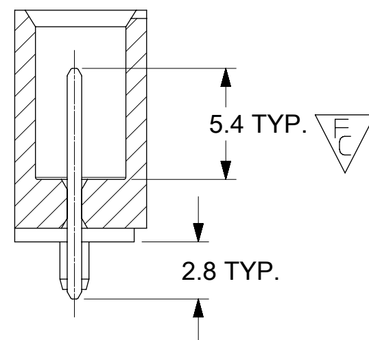
SECTION Z-Z
